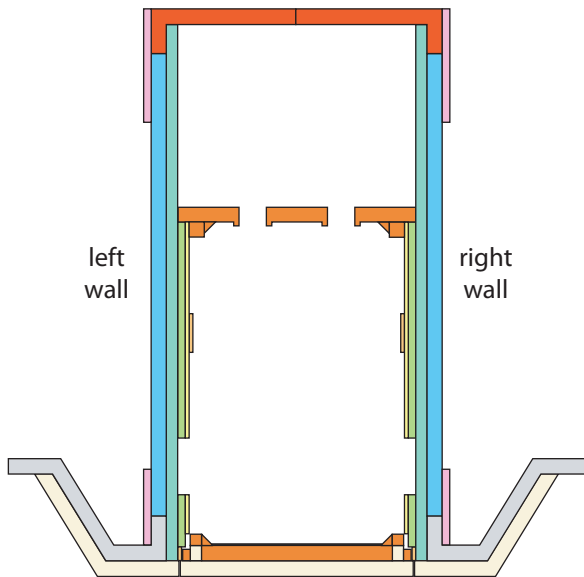
Stack of several styrene sheets (section AA')
